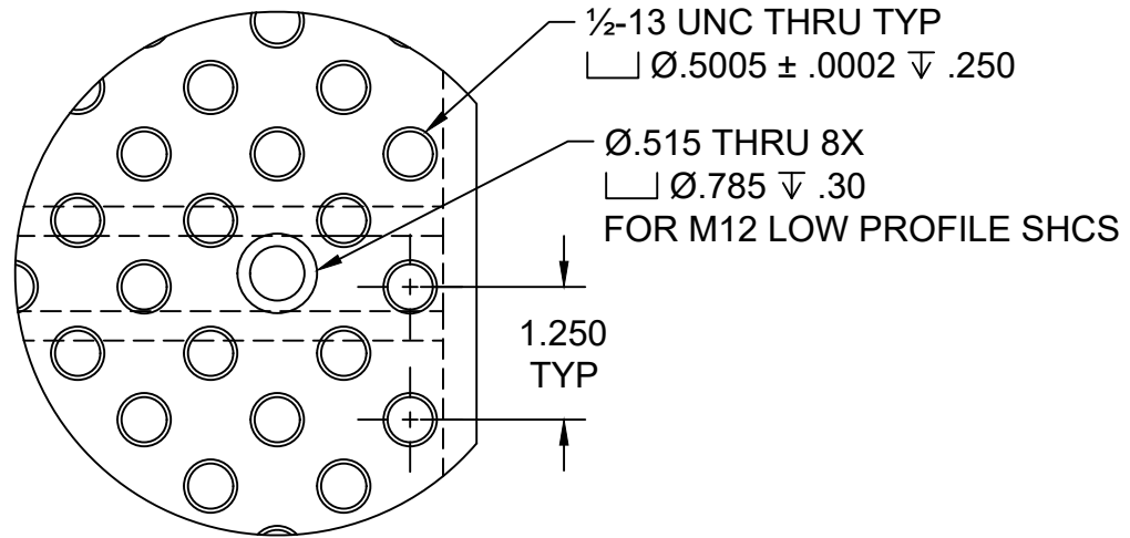
DETAIL A SCALE 1:2
