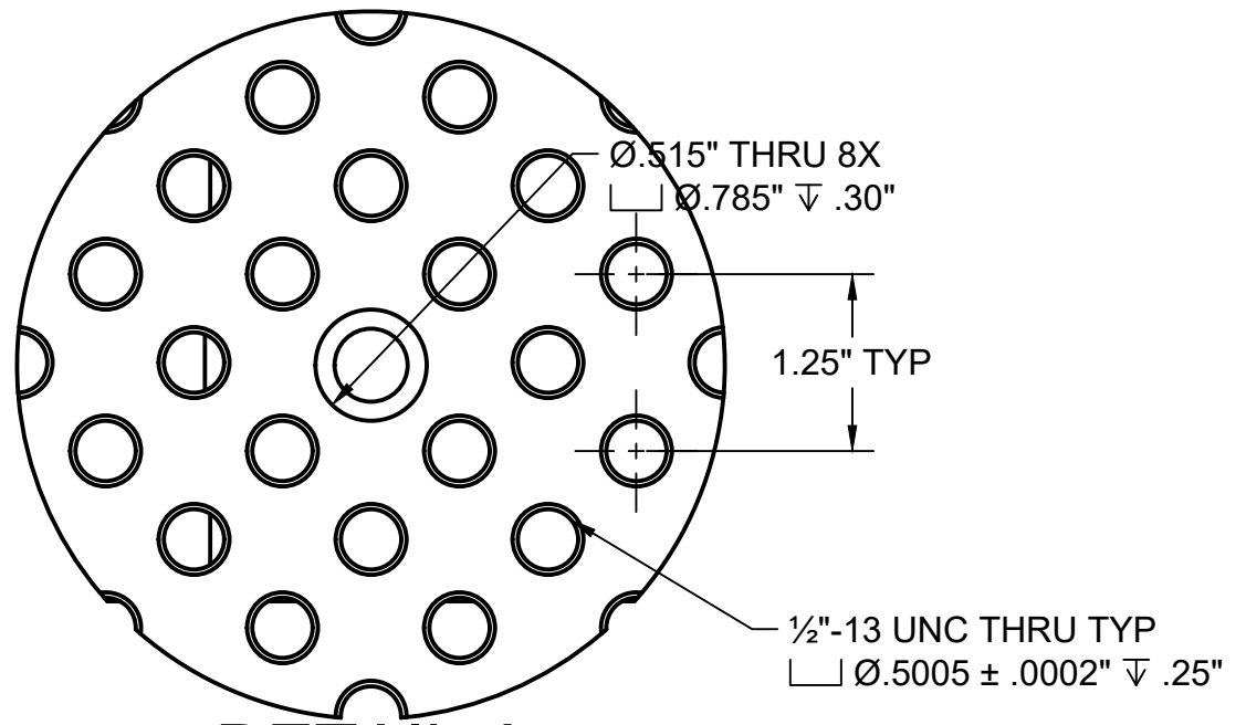
DETAIL A SCALE 2:3
