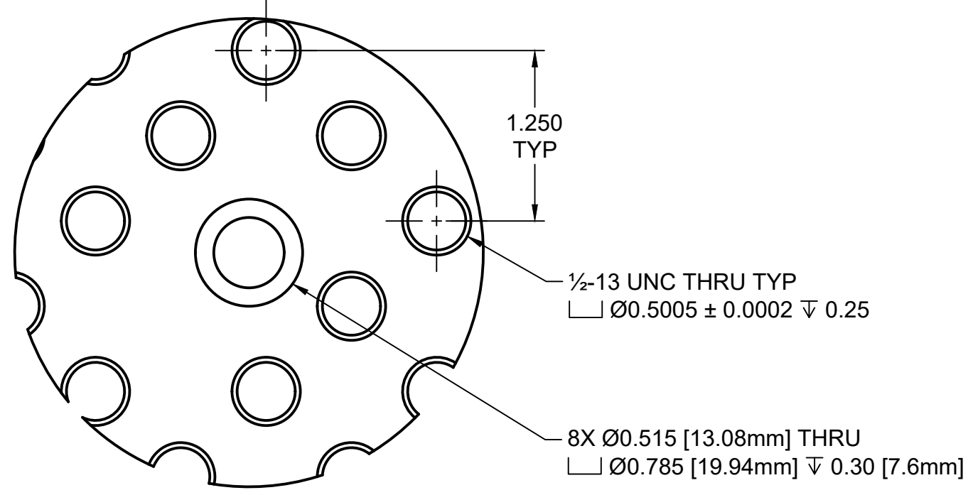
DETAIL A SCALE 1:1
