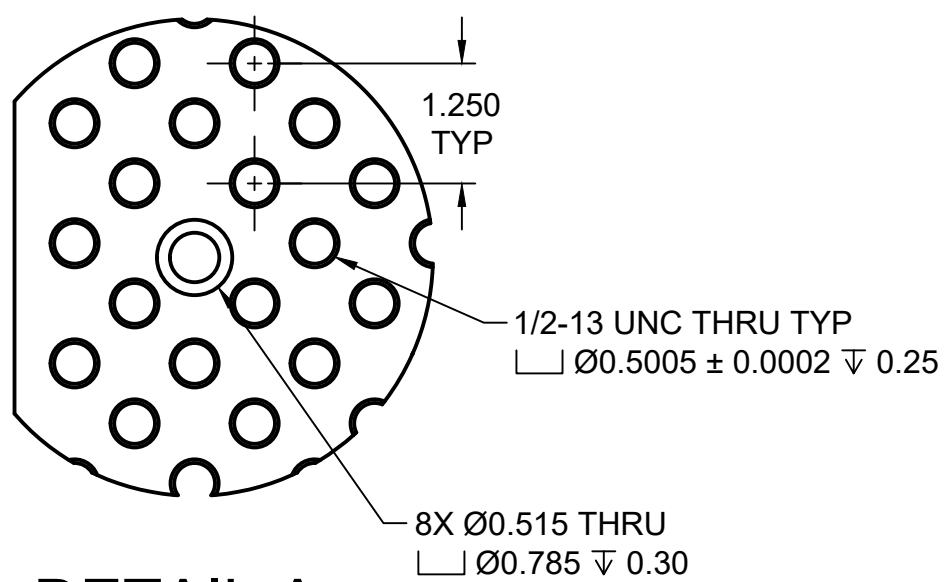
DETAIL A SCALE 1:2
