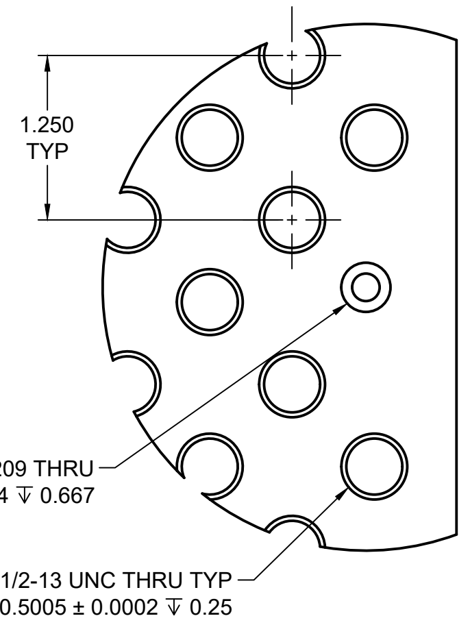
DETAIL A SCALE 1:1
