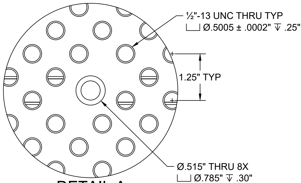
DETAIL A SCALE 2:3
