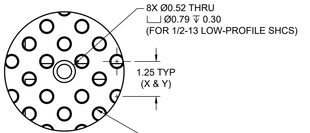
DETAIL B SCALE 1:2
