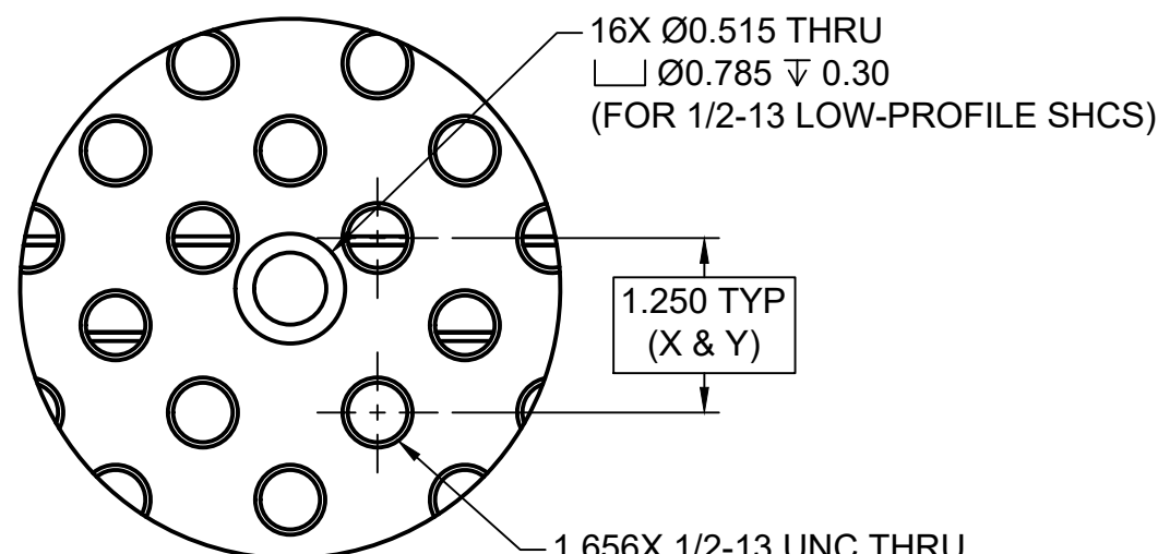
DETAIL A SCALE 2:3
