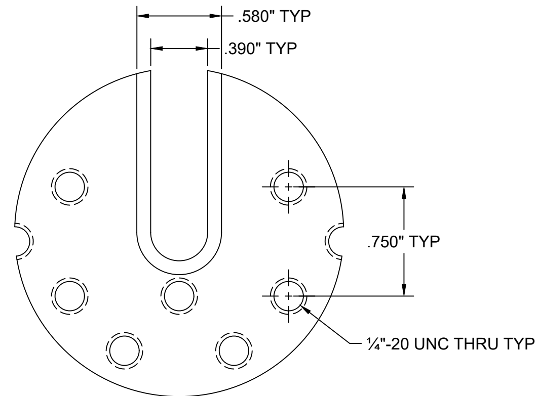
DETAIL B SCALE 3:2
