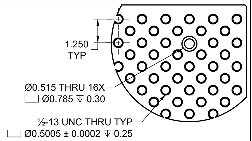
DETAIL A SCALE 1:3
