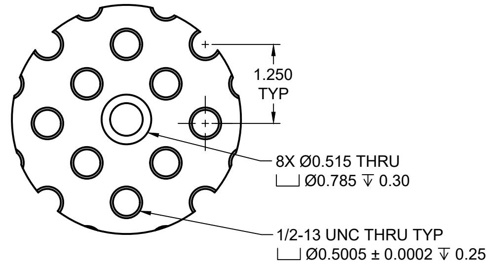
DETAIL A SCALE 2:3
